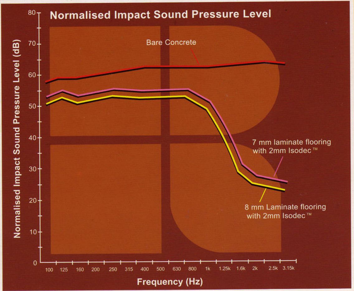
Graph: Impact Isolation of Isodec™ Underlays for Timber Flooring
